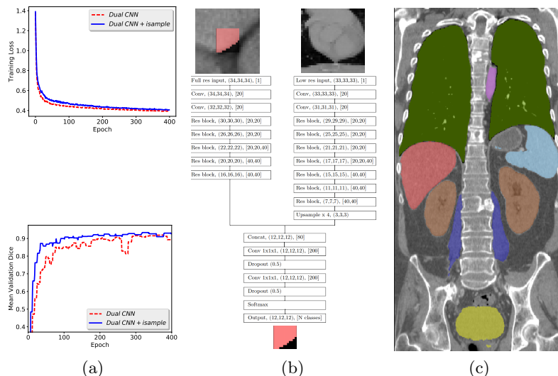
Fig. 1: (a) Training loss (top) and mean validation dice scores (bottom), averaged over 3 runs. (b) The proposed dual path CNN architecture. Numbers inside round brackets give the input dimensions of each block. Numbers in square brackets refer to the number of feature maps used at each layer. (c) Coronal slice of a CT scan with overlaid segmentation output, described in section 3. The organs visible in this slice are: lungs (green), liver (red), spleen (light blue), psoas major muscle (dark blue), kidneys (brown) and bladder (yellow).
